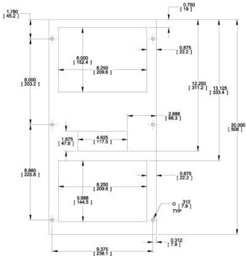
Drilling Template
